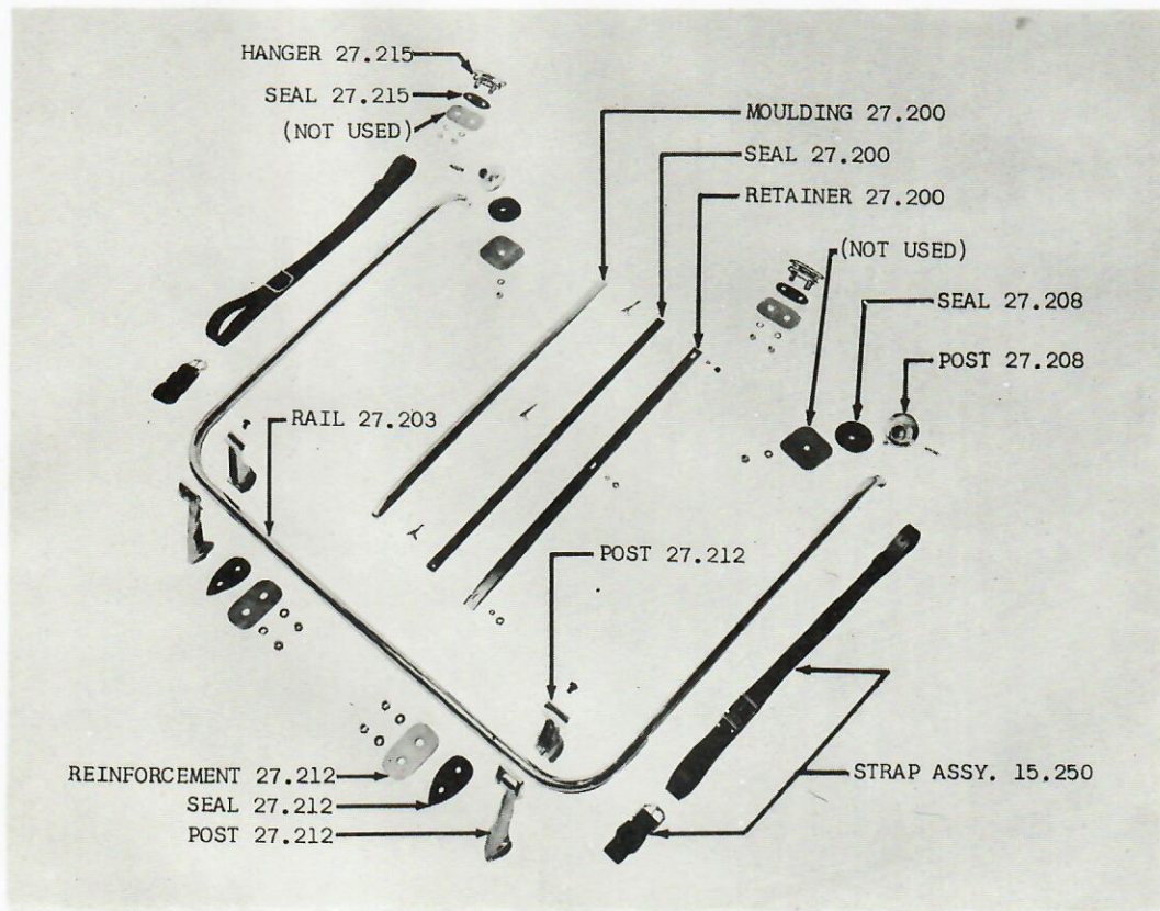
GROUP 27 - FIG. 1 - LUGGAGE RACK 18-28-83-88
